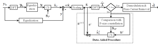
Figure 7: Data-aided compressive sensing implementation at the receiver.
