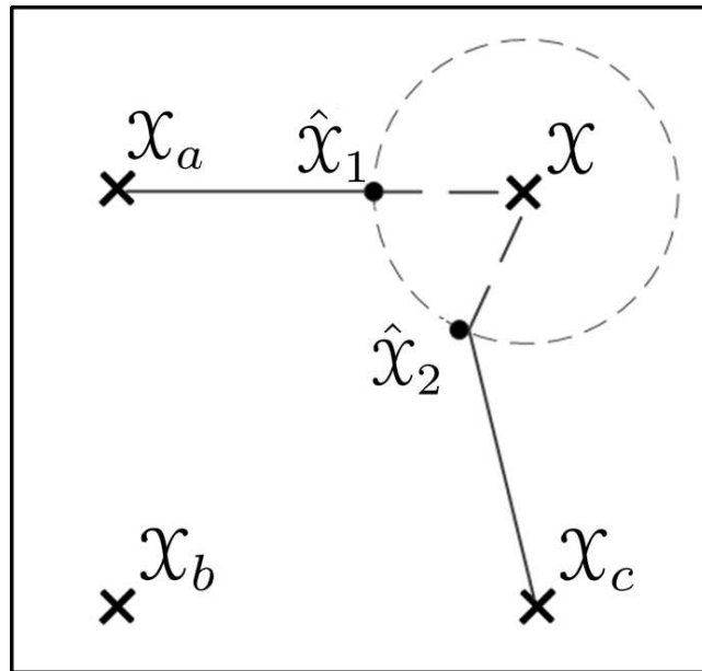
Figure 8: Graphical explanation of the adopted reliability criterion.
