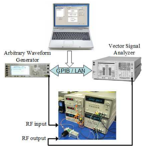
Figure 1: Experimental setup for DUT characterization.
