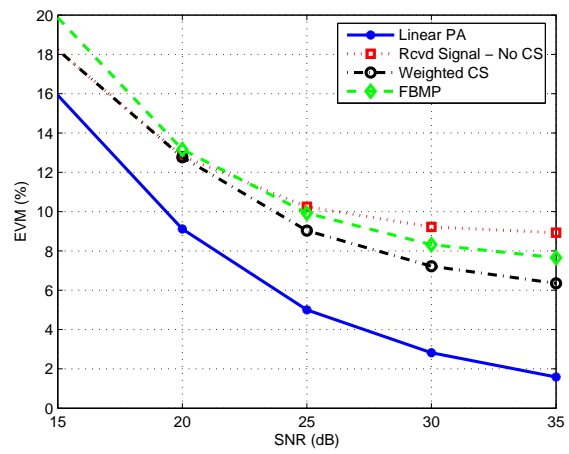
Figure 12: EVM performance comparison of WCS vs. FBMP
